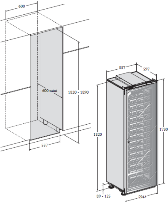
Built-in
