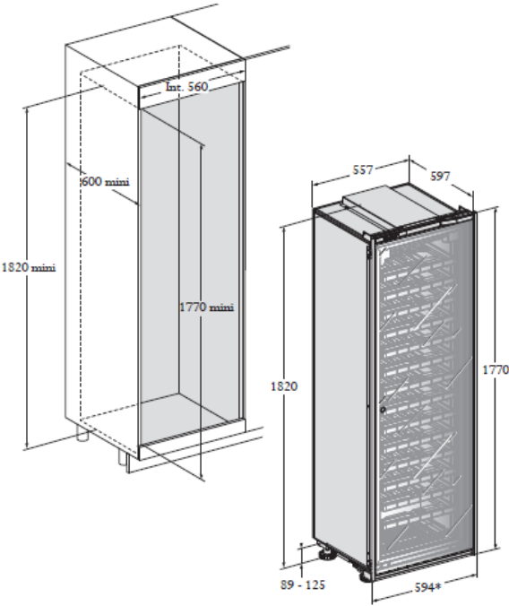
Flush-fitted
